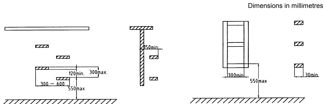
Figure 10 – Boarding means
